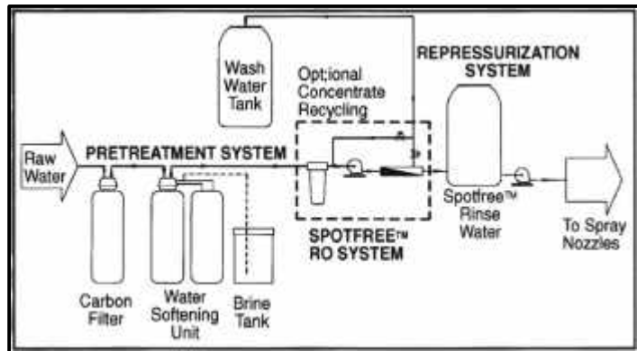
Process Flowchart for Carwash Rinse Water Purification
